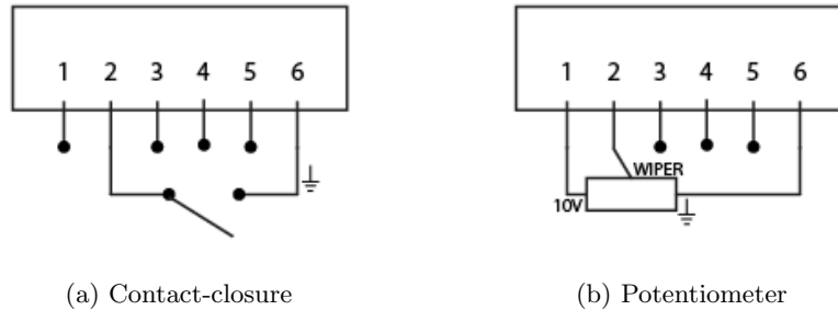
Figure 2.2: GPI Wiring examples
