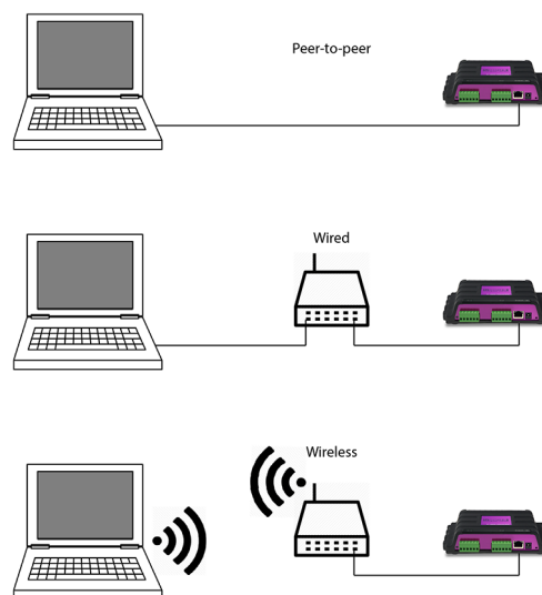
Figure 5.1: Network arrangements
